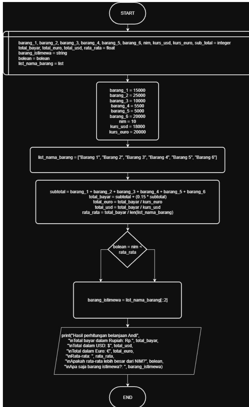
Gambar 1.1 Flowchart Program
